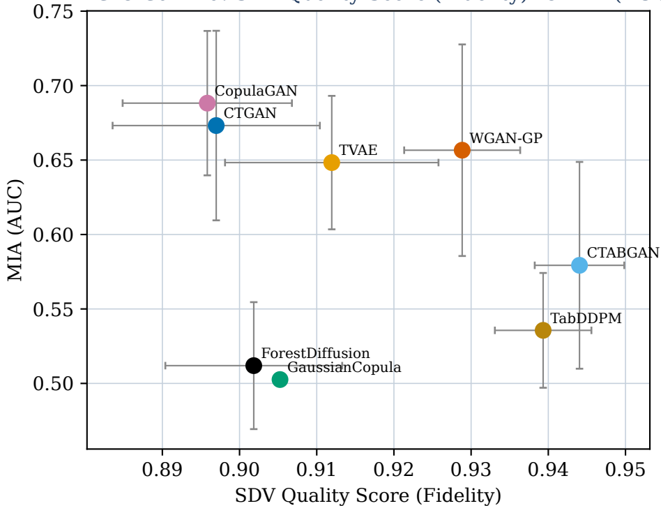
MAGIC Gamma: SDV Quality Score (Fidelity) vs MIA (AUC)
